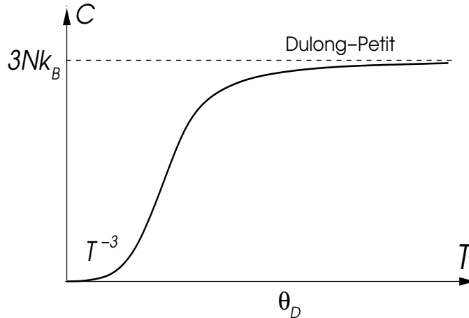
Fig.4.10: heat capacity: Low-temperature behavior follows a T^{-3} -law. At high-temperature the universal Dulong-Petit law recovers, which is a classical result of the equipartition law for particles in a harmonic potential.
