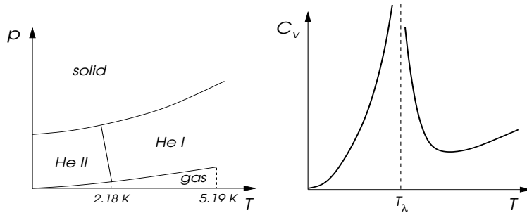
Fig.4.6: ^4\text{He} : Left panel: Schematic phase diagram below 2.18 K the superfluid phase HeII appears and the phase He I is a normal quantum fluid. At 5.19 K a critical end point is located. At high pressure Helium becomes a solid. Right panel: heat capacity shows a singularity at the transition point. Due to the characteristic shape this transition is called "λ-transition".
