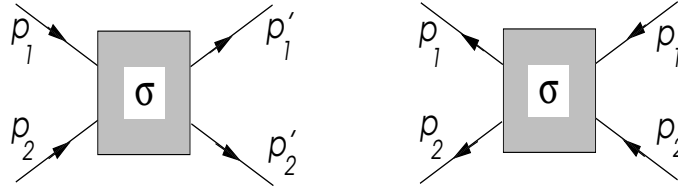
Fig. 2.4: Collision work in both time directions and the matrix elements satisfy a number of symmetry relations.
