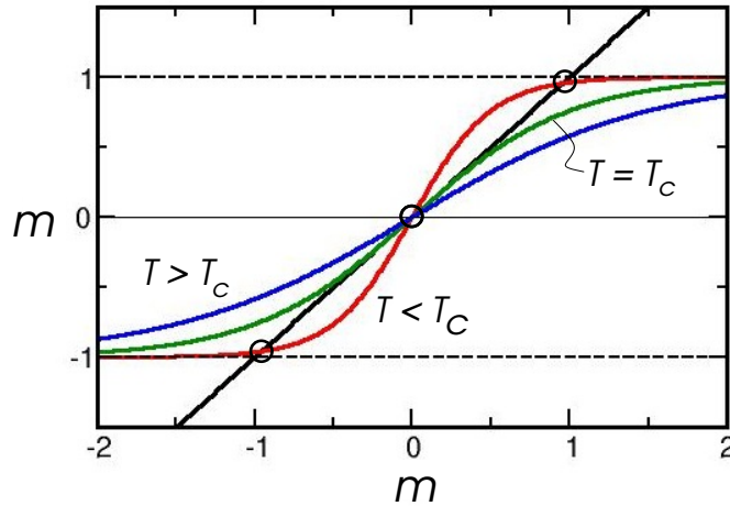
Fig. 5.1: Graphical solution of the self-consistence equation (5.21). The crossing points of the straight line and the step-like function gives the solution. There is only one solution at m = 0 for T \geq T_c and three solutions for T < T_c .
