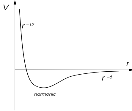
Fig. 3.4: Lennard-Jones potential.
