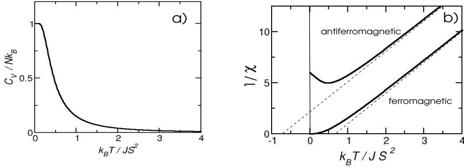
Fig.3.6: Thermodynamic properties of spin chain: a) Specific heat: saturates at low temperature to Nk_B like the potential energy of a two-dimensional harmonic oscillator; b) Susceptibility plotted inversely: ferromagnetic case show divergence at T = 0 and antiferromagnetic case approaches non-monotonically a finite value at T = 0 . Extrapolations from high-temperature region cut horizontal axis at positive (ferromagnetic) and negative (antiferromagnetic) axis, indicating effective energy scales for the corresponding correlations.
