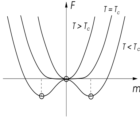
Fig. 5.2: Landau free energy: T > T_c : 2^{\text{nd}} -order term is positive and minimum of F at m = 0 ; T = T_c , 2^{\text{nd}} vanishes and free energy minimum at m = 0 becomes very shallow; T < T_c : 2^{\text{nd}} -order term is negative and minimum of F is at finite value of m , bounded by the 4^{\text{th}} -order term.
