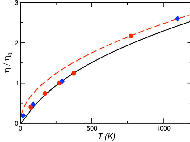
Fig. 2.5: Viscosity for He and H 2 renormalized with \eta_0 ( \eta_0^{(He)} = 18.85 \times 10^{-6} \text{kgm}^{-1}\text{s}^{-1} and \eta_0^{(H_2)} = 8.4 \times 10^{-6} \text{kgm}^{-1}\text{s}^{-1} ). The solid line corresponds to Sutherlands formula and the dashes line is the \sqrt{T} -law. The experimental data are given for Helium (diamonds) and H 2 (circles).
