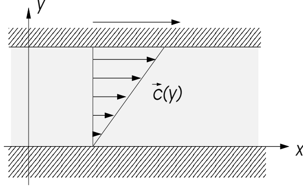
Fig. 2.4: Velocity profile between two moving plates.
