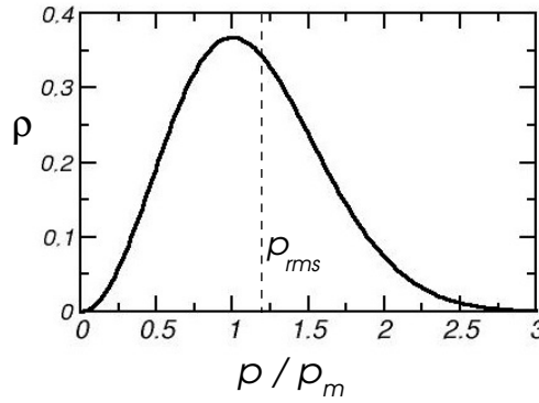
Fig. 2.3: Momentum distribution of an ideal gas in equilibrium. Maximal ( p_m ) and root-mean-square momentum ( p_{rms} ) are not identical.
