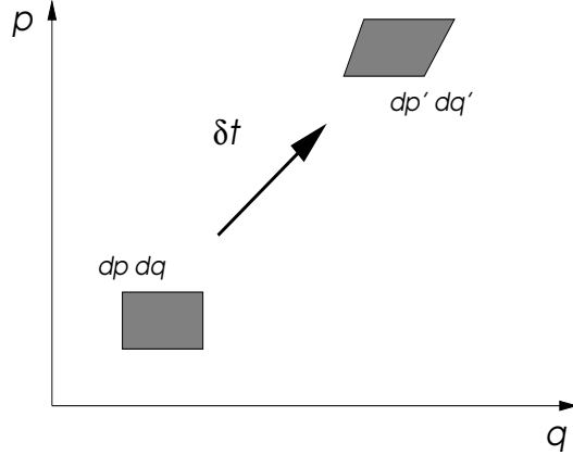
Fig. 2.1: Temporal evolution of the phase space volume d^3p d^3q .
