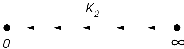
Fig.7.2: Flow of the coupling constant K_2 = J/k_B T of the one-dimensional Ising model under the renormalization group scheme. For any finite coupling and temperature the flow goes towards K = 0 the limit of completely decoupled spins.
