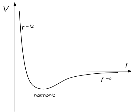
Fig. 3.4: Lenard-Jones potential.
