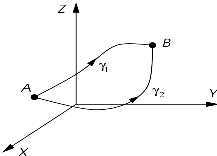
Fig.1.1: Space of states: A and B are equilibrium states connected by paths \gamma_1 or \gamma_2 .
