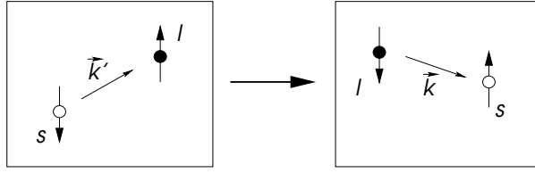
Fig. 2.7: Spin exchange scattering of an electron at a nuclear spin I .
