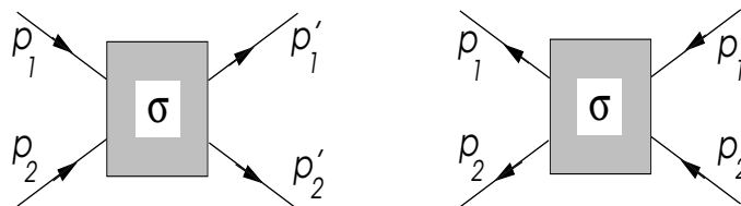
Fig. 2.2: Collision work in both time directions and the matrix elements satisfy a number of symmetry relations.
